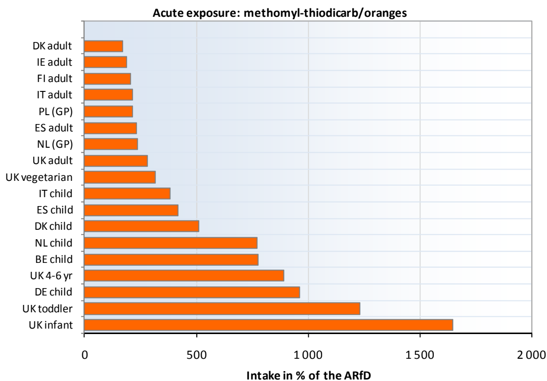
Figure 5.2.14-3: Acute exposure of the European population to methomyl/thiodicarb residues in oranges, expressed as percent of the ARfD set for methomyl.
