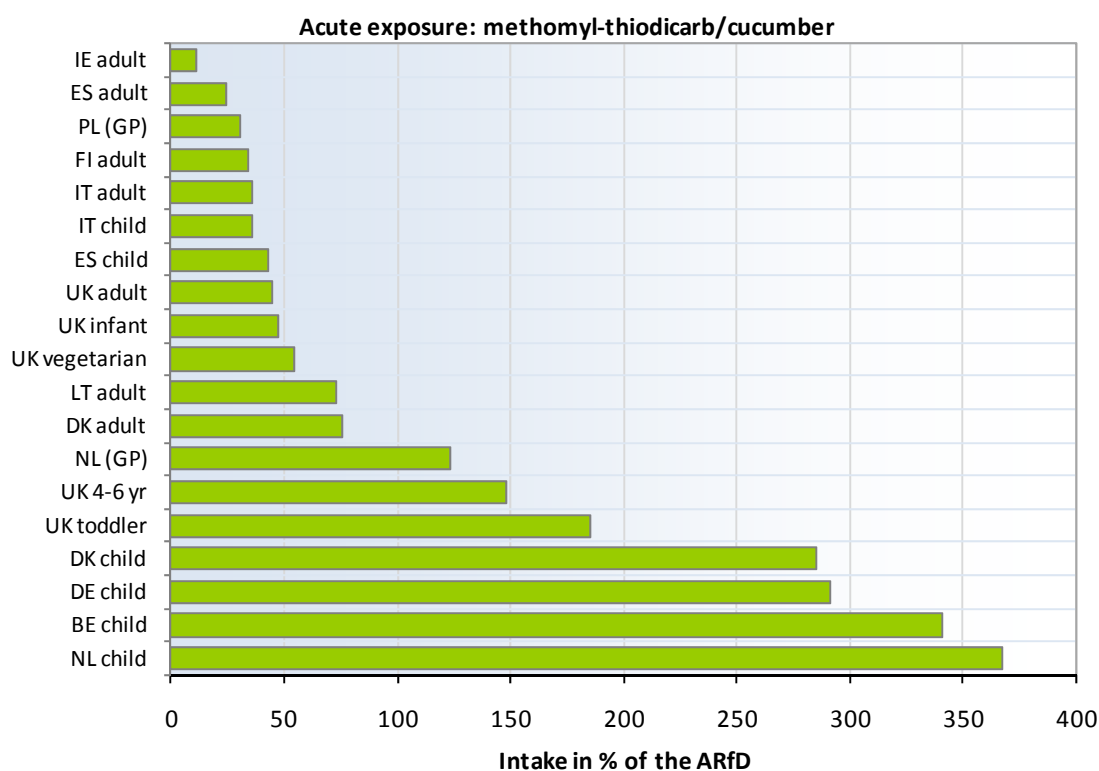
Figure 5.2.14-2: Acute exposure of the European population to methomyl/thiodicarb residues in cucumbers, expressed as percent of the ARfD set for methomyl.
